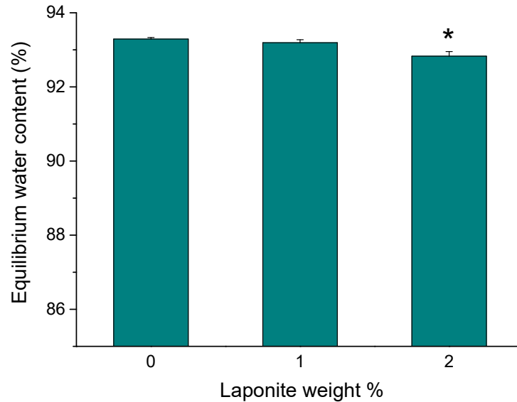
Figure 3.6 Equilibrium water content of PEG-D4 hydrogels cured using a \text{NaIO}_4 :dopamine molar ratio of 0.5 and Laponite content of 0-2 wt%. * p < 0.05 when compared to 0 wt% Laponite.
