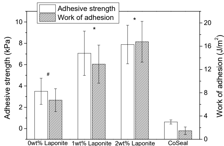
Figure 3.10 Lap shear adhesion test results of PEG-D4 hydrogels with NaIO 4 :dopamine molar ratio of 0.5 containing up to 2 wt% Laponite. * p < 0.05 when compared to 0 wt% Laponite and CoSeal. # p < 0.05 when compared to CoSeal.
