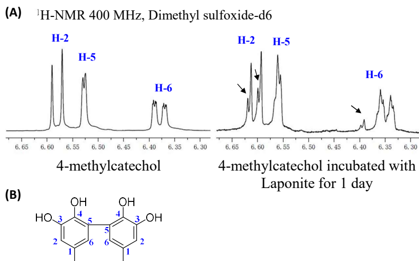
Figure 4.4 (A) 1 H NMR spectra of catecholic benzene ring region of 4-methylcatechol and 4-methylcatechol incubated with Laponite for 1 day. The partial peak separations of the 1 H linked to C-2 and C-6 (arrows) suggested that the new covalent bonds occurred to C5 [213]. A relative decrease in the peak area for H-5 (from 1.01 to 0.9 when a reference integral value of 1 for H-2 was set) was observed. (B) The proposed structure of dimerized 4-methylcatechol.
