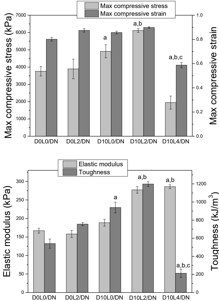
Figure 2.3 Measured compressive strength, strain, elastic modulus, and toughness of DN hydrogels. Data were presented as mean \pm SD (n = 3). a p < 0.05 when compared to D0L0/DN and D0L2/DN, b p < 0.05 when compared to D10L0/DN, c p < 0.05 when compared to D10L2/DN.
