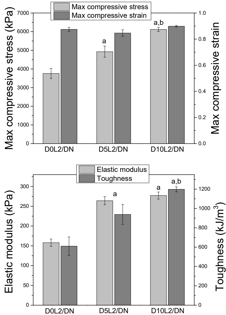
Figure 2.4 Measured compressive strength, strain, elastic modulus, and toughness of DN hydrogels. Data were presented as mean \pm SD ( n = 3 ). a p < 0.05 when compared to D0L2/DN, b p < 0.05 when compared to D5L2/DN.
